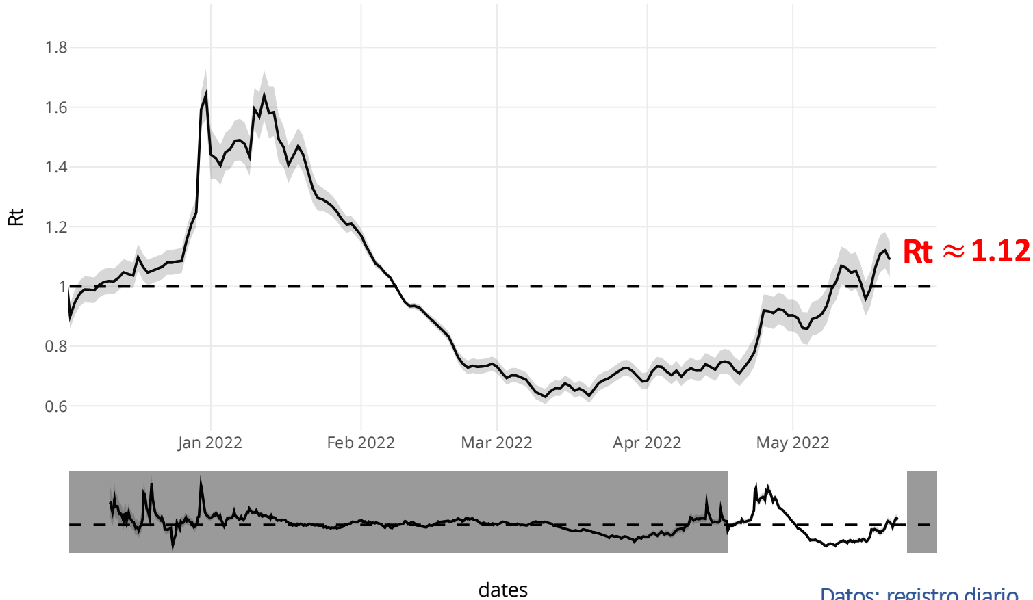
Paraguay - R instantaneo: Mean(R), Q 0.05, Q 0.95; 2020-03-07 - 2022-05-21
