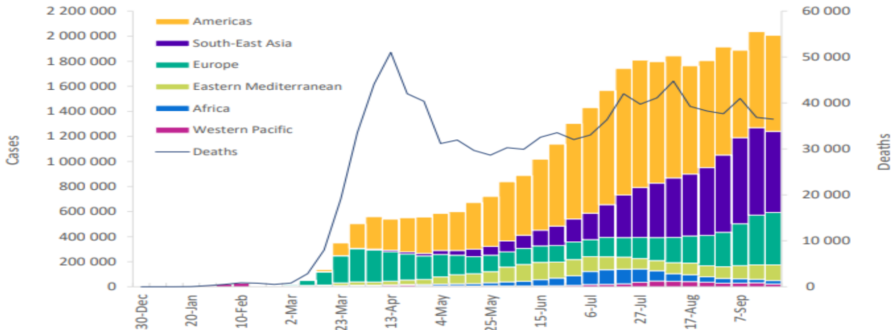
Figure 1: Number of COVID-19 cases reported weekly by WHO Region, and global deaths, 30 December 2019 through 27 September 2020**
