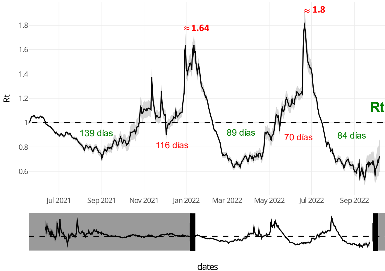
Paraguay - R instantaneo: Mean(R), Q 0.05, Q 0.95; 2020-03-07 - 2022-10-08
